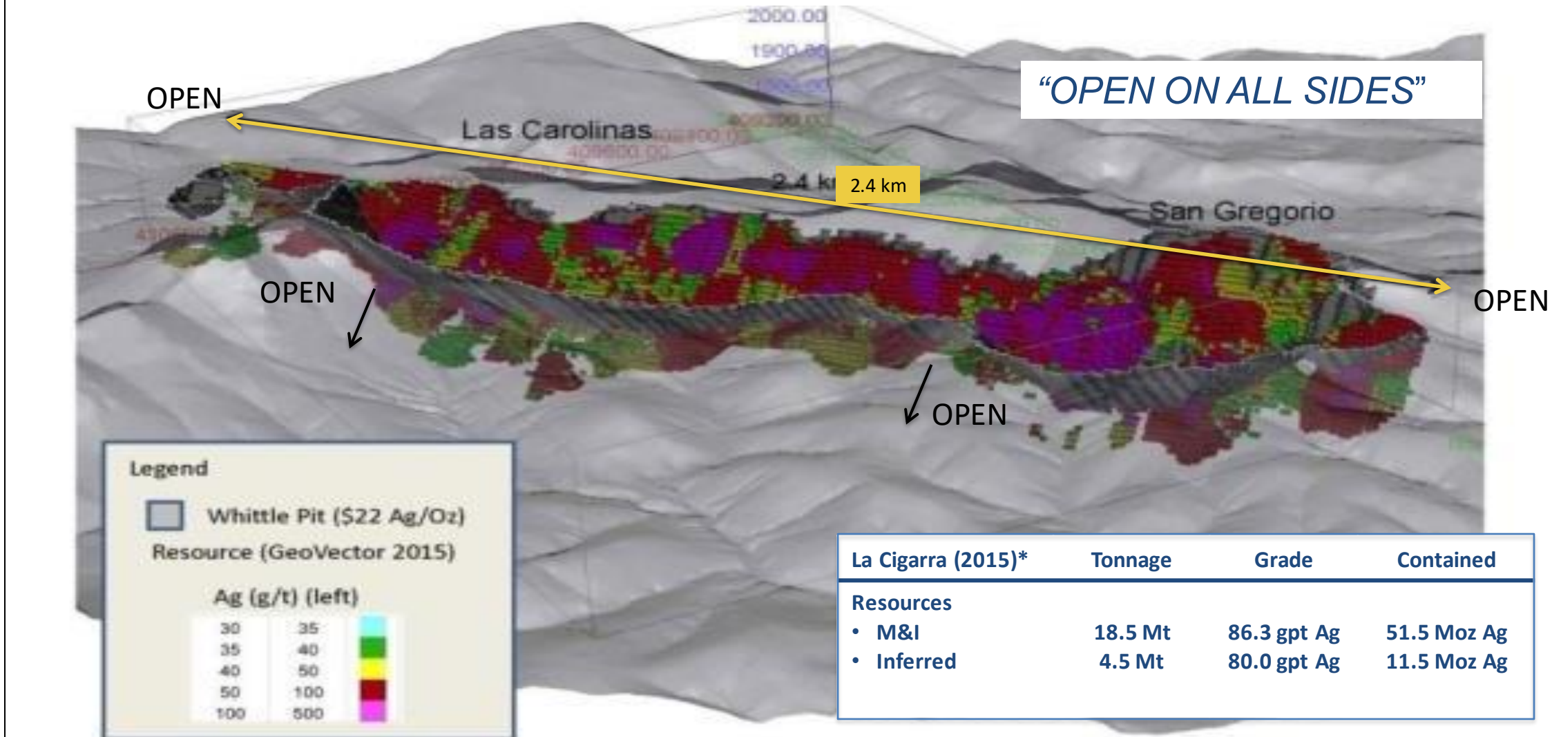
3D view looking southwest of the San Gregorio/Las Carolina resource blocks (>35 gpt Ag) Whittle pit ($22 Ag/Oz)
